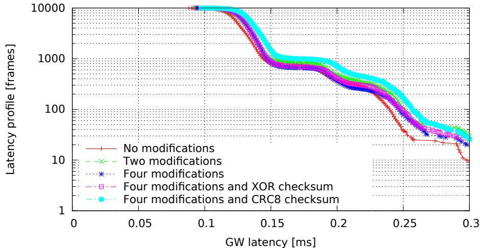
Single GW rule for all messages with modifications, 8 byte messages (GW kernel 3.0.7-rt20-00008-g0c18035, Traffic onetatime, Load cpu)
