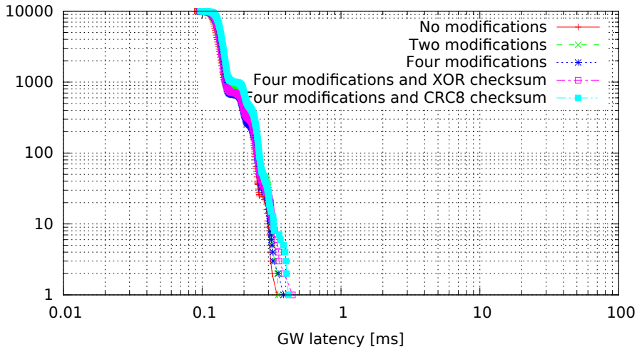
Single GW rule for all messages with modifications, 8 byte messages (GW kernel 3.0.7-rt20-00008-g0c18035, Traffic oneatatime, Load cpu)
