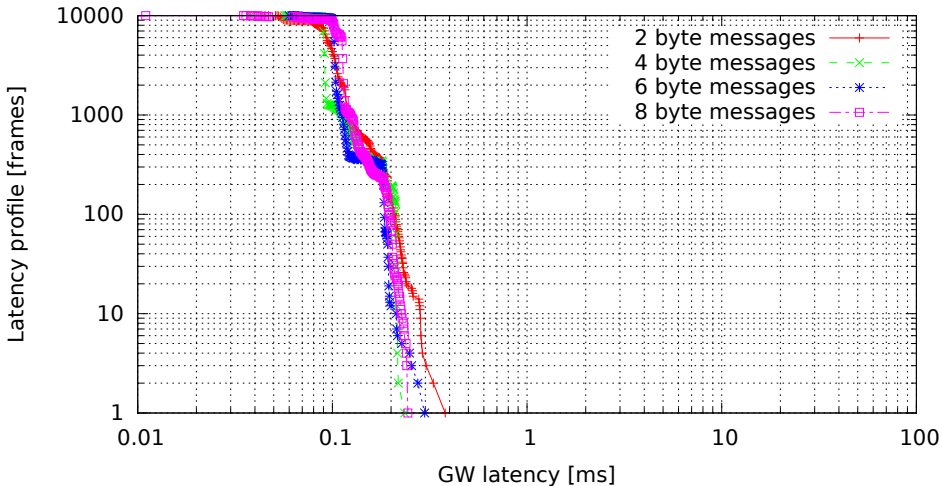
Single GW rule for all messages, no modifications, high (soft)irq task priority (GW kernel 3.0.7-rt20-00008-g0c18035, Traffic flood, Load none)
