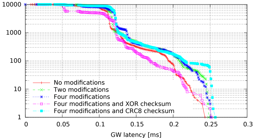
Single GW rule for all messages with modifications, 8 byte messages (GW kernel 3.0.7-rt20-00008-g0c18035, Traffic flood, Load none)
