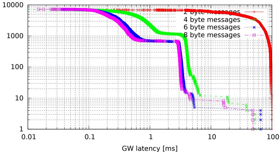
Single GW rule for all messages, no modifications (GW kernel 3.0.7-rt20-00008-g0c18035, Traffic flood, Load eth)
