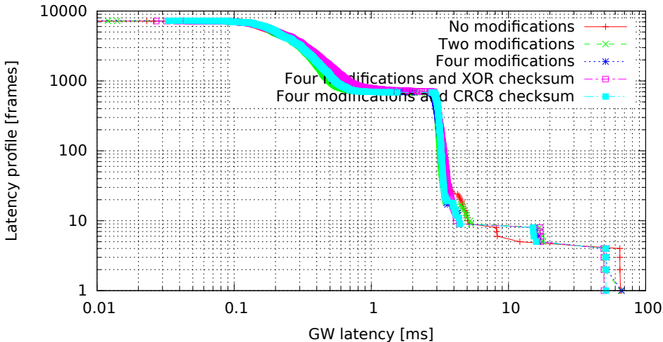
Single GW rule for all messages with modifications, 8 byte messages (GW kernel 3.0.7-rt20-00008-g0c18035, Traffic flood, Load eth)
