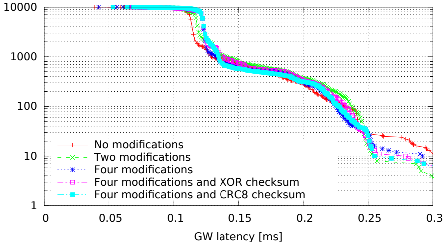
Single GW rule for all messages with modifications, 8 byte messages (GW kernel 3.0.7-rt20-00008-g0c18035, Traffic flood, Load cpu)
