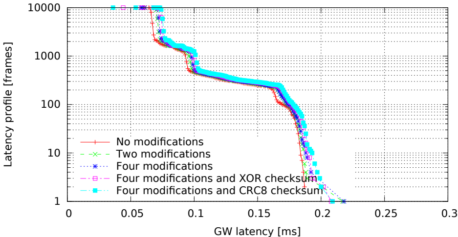
Single GW rule for all messages with modifications, 8 byte messages (GW kernel 3.0.7-rt20-00008-g0c18035, Traffic 50, Load none)
