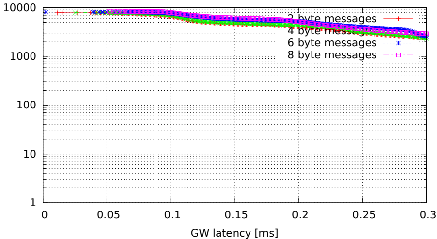
Single GW rule for all messages, no modifications (GW kernel 3.0.7-rt20-00008-g0c18035, Traffic 50, Load eth)
