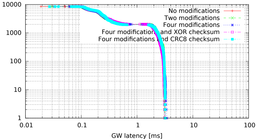
Single GW rule for all messages with modifications, 8 byte messages (GW kernel 3.0.7-rt20-00008-g0c18035, Traffic 50, Load eth)
