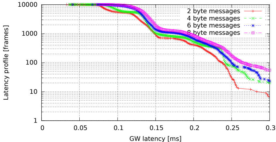
Single GW rule for all messages, no modifications (GW kernel 3.0.7-rt20-00008-g0c18035, Traffic 50, Load cpu)
