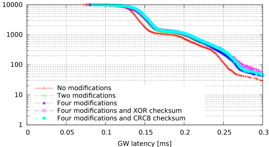
Single GW rule for all messages with modifications, 8 byte messages (GW kernel 3.0.7-rt20-00008-g0c18035, Traffic 50, Load cpu)
