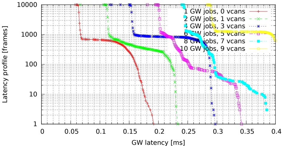
Chained GWs on multiple VCAN interfaces (GW kernel 3.0.4-rt14-00008-gb2052fd, Traffic onetatime, Load none)
