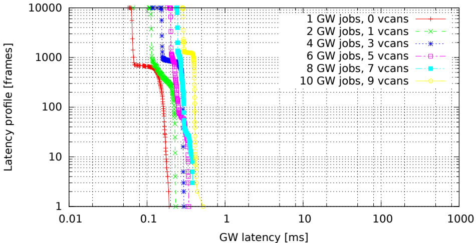
Chained GWs on multiple VCAN interfaces (GW kernel 3.0.4-rt14-00008-gb2052fd, Traffic oneatatime, Load none)
