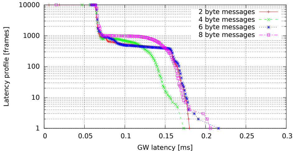
Single GW rule for all messages, no modifications (GW kernel 3.0.4-rt14-00008-gb2052fd, Traffic oneatatime, Load none)
