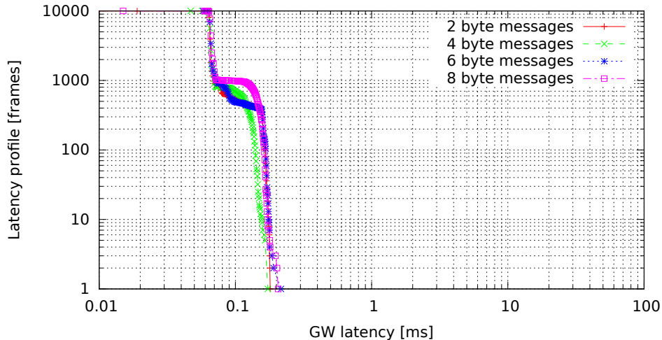
Single GW rule for all messages, no modifications (GW kernel 3.0.4-rt14-00008-gb2052fd, Traffic onetatime, Load none)
