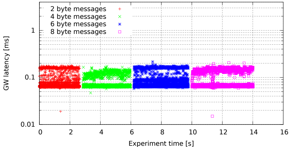
Single GW rule for all messages, no modifications (GW kernel 3.0.4-rt14-00008-gb2052fd, Traffic oneatatime, Load none)
