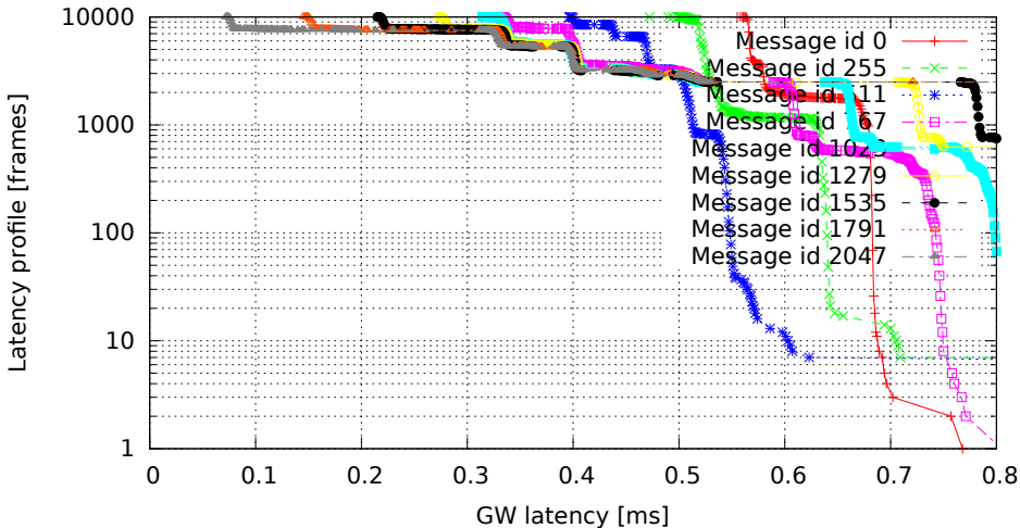
2048 GW rules (one per id, mask 0x7FF), no modifications (GW kernel 3.0.4-rt14-00008-gb2052fd, Traffic onetatime, Load none)
