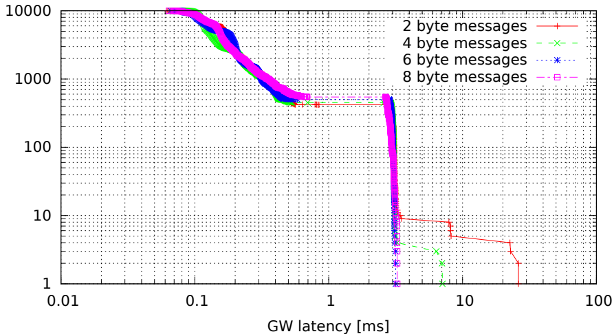
Single GW rule for all messages, no modifications (GW kernel 3.0.4-rt14-00008-gb2052fd, Traffic oneatatime, Load eth)
