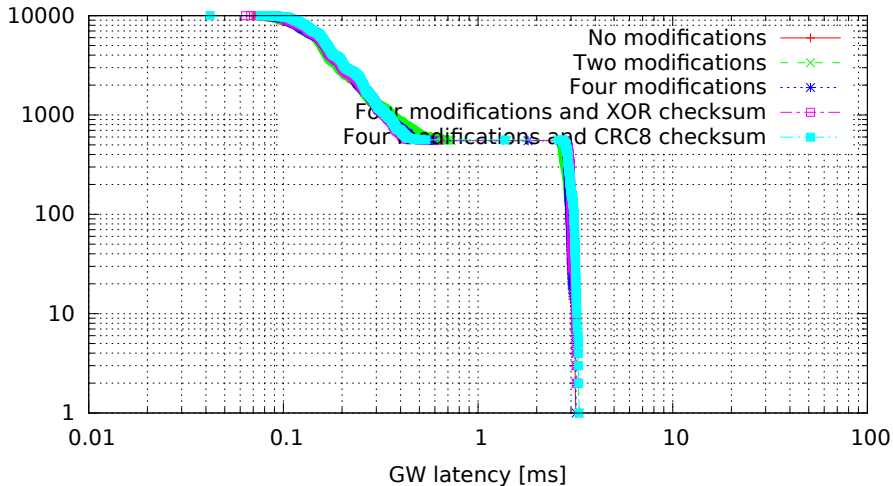
Single GW rule for all messages with modifications, 8 byte messages (GW kernel 3.0.4-rt14-00008-gb2052fd, Traffic onetatime, Load eth)
