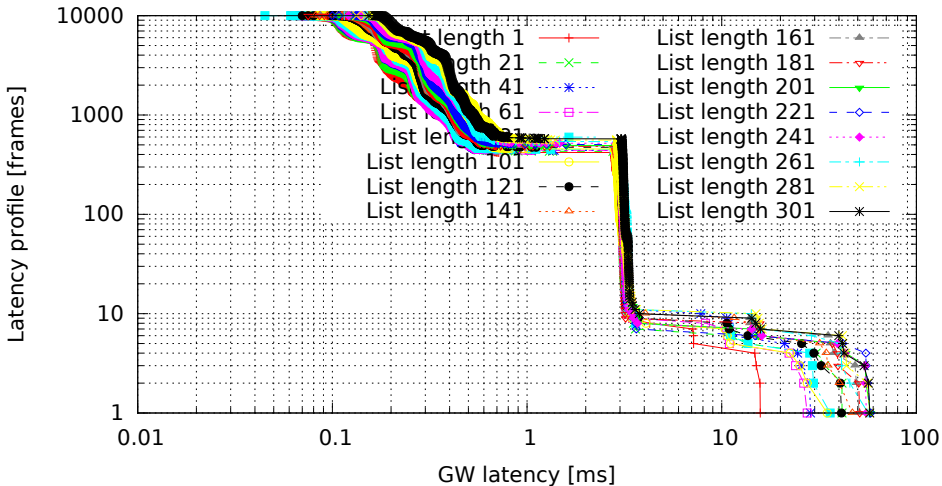
Different lengths of filter list, only the last one matches (GW kernel 3.0.4-rt14-00008-gb2052fd, Traffic oneatatime, Load eth)
