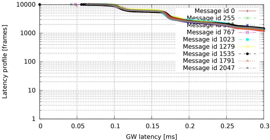
2048 GW rules (one per id, mask C00007FF), no modifications (GW kernel 3.0.4-rt14-00008-gb2052fd, Traffic oneatatime, Load eth)
