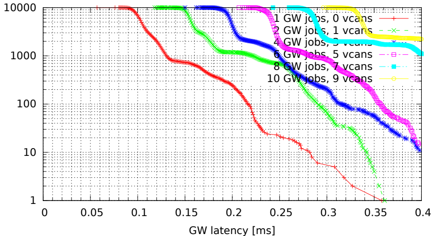
Chained GWs on multiple VCAN interfaces (GW kernel 3.0.4-rt14-00008-gb2052fd, Traffic oneatatime, Load cpu)
