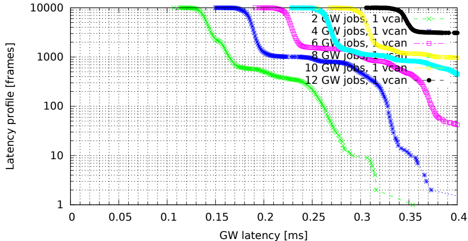
Chained GWs on a single VCAN interface (GW kernel 3.0.4-rt14-00008-gb2052fd, Traffic oneatatime, Load cpu)
