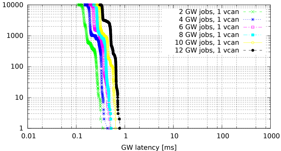
Chained GWs on a single VCAN interface (GW kernel 3.0.4-rt14-00008-gb2052fd, Traffic oneatatime, Load cpu)
