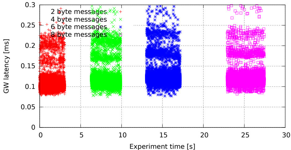
Single GW rule for all messages, no modifications (GW kernel 3.0.4-rt14-00008-gb2052fd, Traffic oneatatime, Load cpu)
