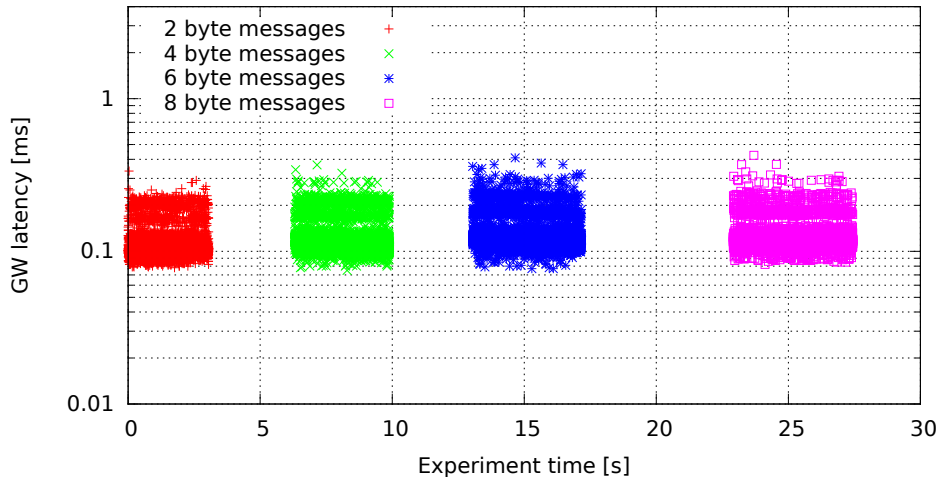
Single GW rule for all messages, no modifications (GW kernel 3.0.4-rt14-00008-gb2052fd, Traffic oneatatime, Load cpu)
