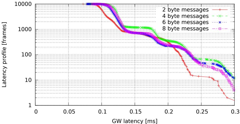
Single GW rule for all messages, no modifications, high (soft)irq task priority (GW kernel 3.0.4-rt14-00008-gb2052fd, Traffic oneatatime, Load cpu)
