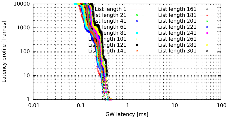
Different lengths of filter list, only the last one matches (GW kernel 3.0.4-rt14-00008-gb2052fd, Traffic oneatatime, Load cpu)
