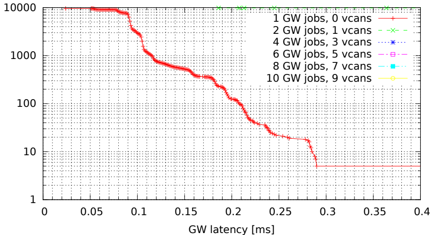
Chained GWs on multiple VCAN interfaces (GW kernel 3.0.4-rt14-00008-gb2052fd, Traffic flood, Load none)
