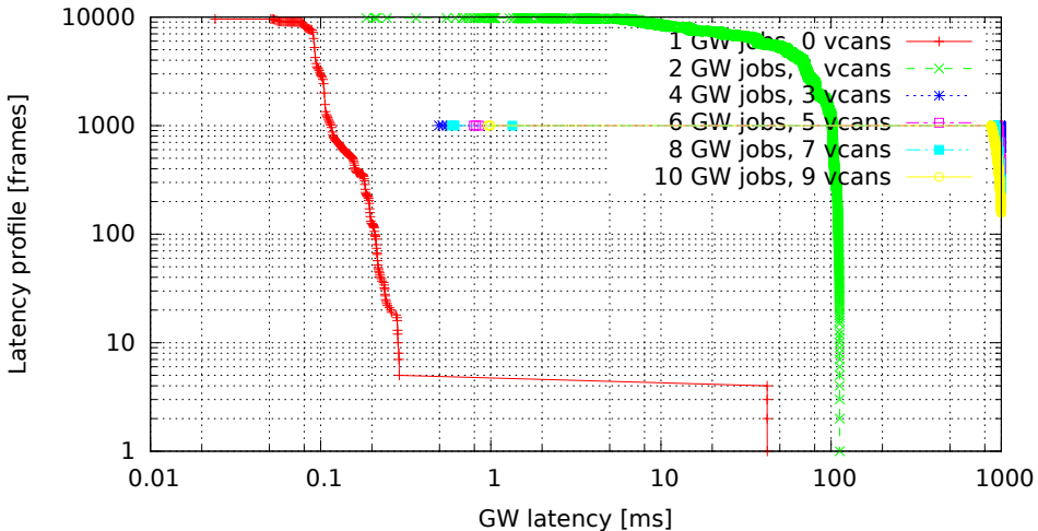
Chained GWs on multiple VCAN interfaces (GW kernel 3.0.4-rt14-00008-gb2052fd, Traffic flood, Load none)
