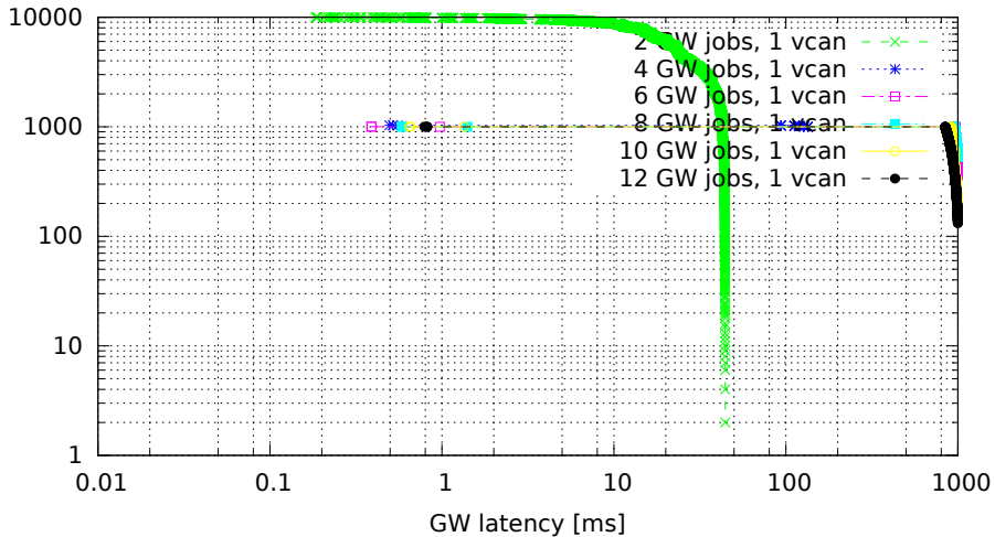
Chained GWs on a single vcan interface (GW kernel 3.0.4-rt14-00008-gb2052fd, Traffic flood, Load none)
