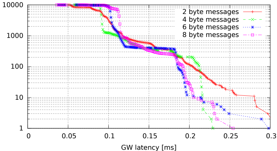
Single GW rule for all messages, no modifications (GW kernel 3.0.4-rt14-00008-gb2052fd, Traffic flood, Load none)
