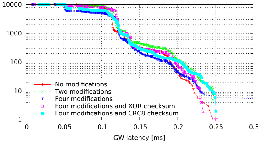
Single GW rule for all messages with modifications, 8 byte messages (GW kernel 3.0.4-rt14-00008-gb2052fd, Traffic flood, Load none)
