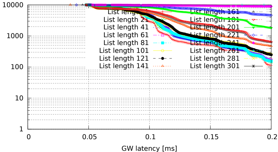
Different lengths of filter list, only the last one matches (GW kernel 3.0.4-rt14-00008-gb2052fd, Traffic flood, Load none)
