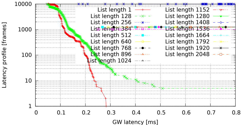
Different lengths of filter list, only the last one matches (GW kernel 3.0.4-rt14-00008-gb2052fd, Traffic flood, Load none)
