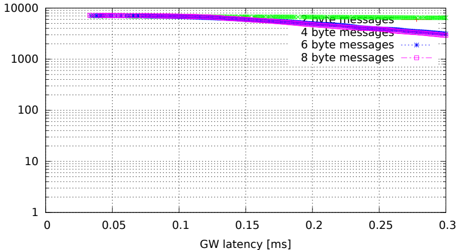
Single GW rule for all messages, no modifications (GW kernel 3.0.4-rt14-00008-gb2052fd, Traffic flood, Load eth)
