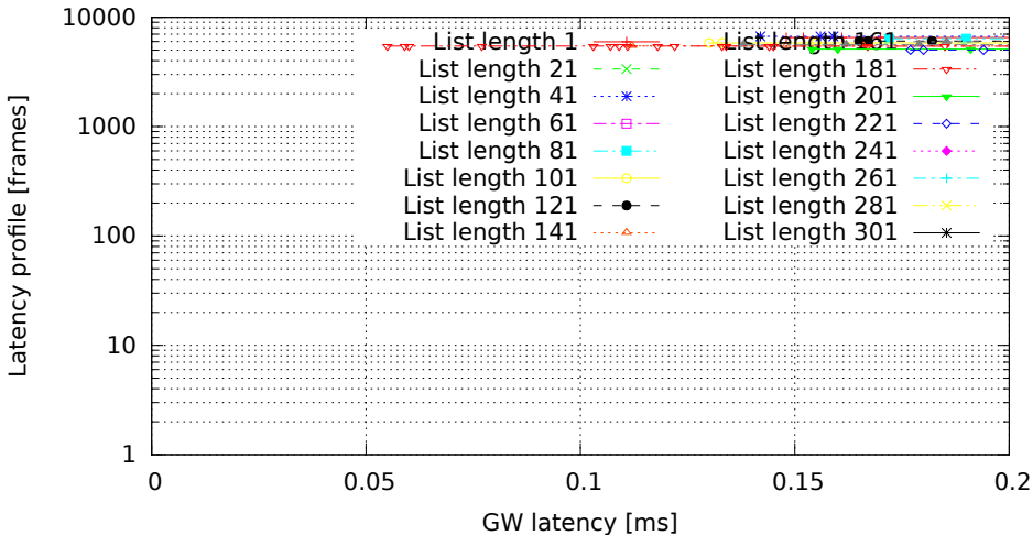
Different lengths of filter list, only the last one matches (GW kernel 3.0.4-rt14-00008-gb2052fd, Traffic flood, Load eth)
