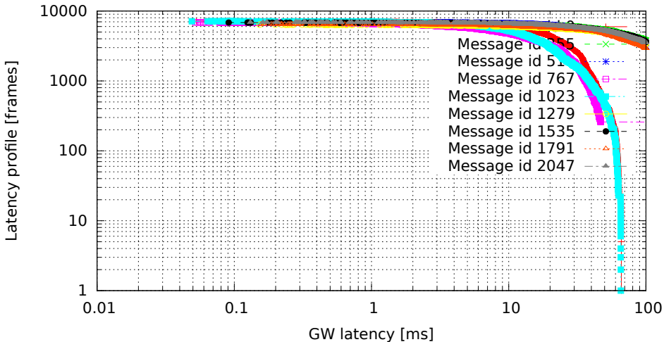
2048 GW rules (one per id, mask C00007FF), no modifications (GW kernel 3.0.4-rt14-00008-gb2052fd, Traffic flood, Load eth)
