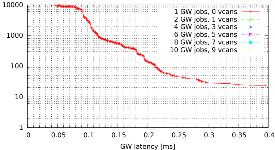
Chained GWs on multiple VCAN interfaces (GW kernel 3.0.4-rt14-00008-gb2052fd, Traffic flood, Load cpu)
