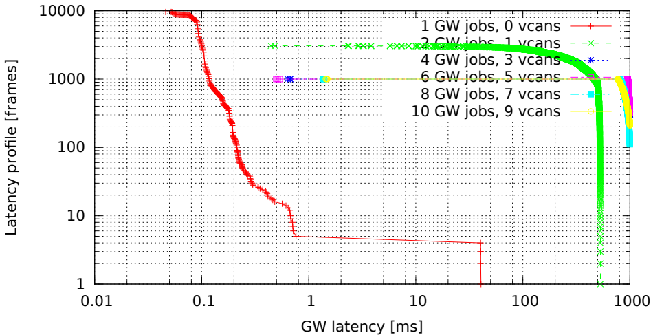
Chained GWs on multiple VCAN interfaces (GW kernel 3.0.4-rt14-00008-gb2052fd, Traffic flood, Load cpu)
