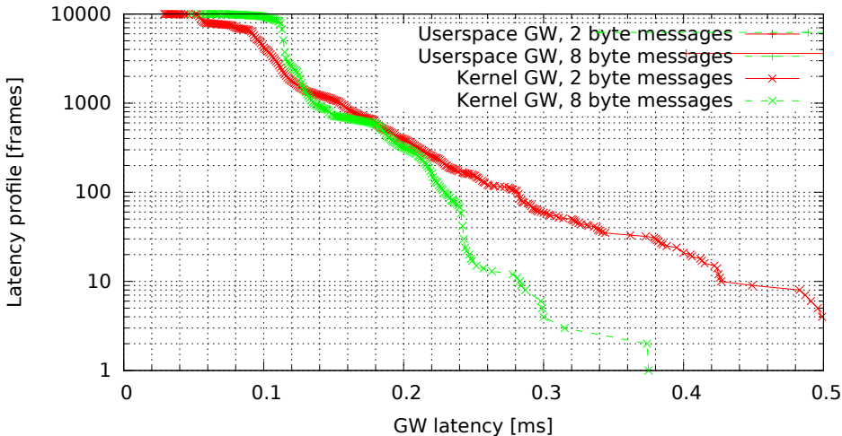
Kernel vs. userspace GW, no modifications (GW kernel 3.0.4-rt14-00008-gb2052fd, Traffic flood, Load cpu)
