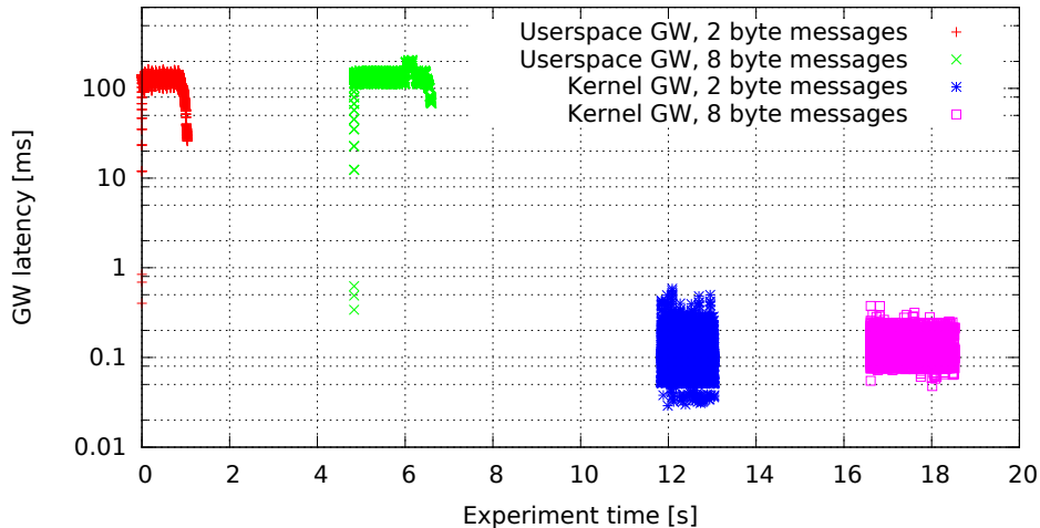
Single GW rule for all messages, no modifications (GW kernel 3.0.4-rt14-00008-gb2052fd, Traffic flood, Load cpu)
