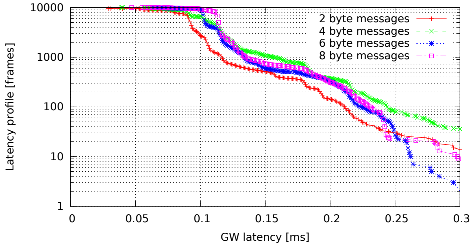
Single GW rule for all messages, no modifications (GW kernel 3.0.4-rt14-00008-gb2052fd, Traffic flood, Load cpu)
