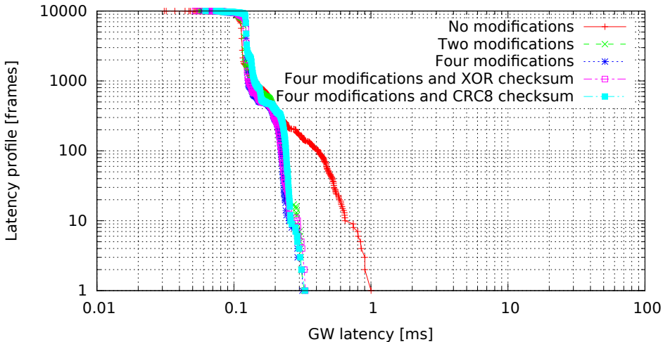
Single GW rule for all messages with modifications, 8 byte messages (GW kernel 3.0.4-rt14-00008-gb2052fd, Traffic flood, Load cpu)
