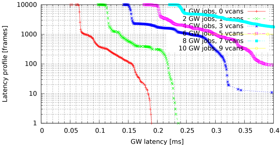
Chained GWs on multiple VCAN interfaces (GW kernel 3.0.4-rt14-00008-gb2052fd, Traffic 50, Load none)
