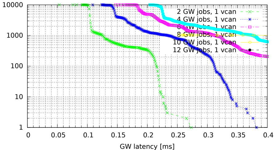
Chained GWs on a single VCAN interface (GW kernel 3.0.4-rt14-00008-gb2052fd, Traffic 50, Load none)
