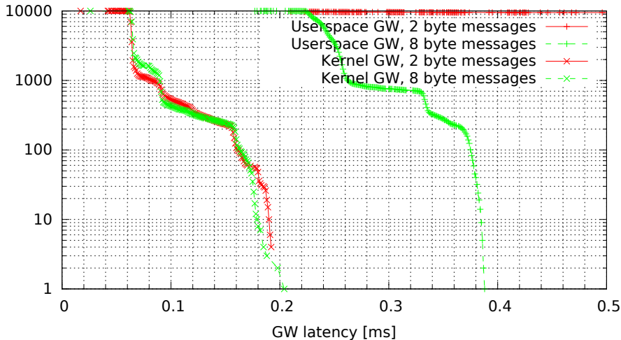
Kernel vs. userspace GW, no modifications (GW kernel 3.0.4-rt14-00008-gb2052fd, Traffic 50, Load none)
