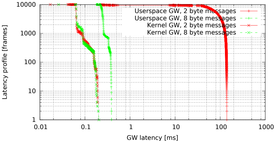
Kernel vs. userspace GW, no modifications (GW kernel 3.0.4-rt14-00008-gb2052fd, Traffic 50, Load none)
