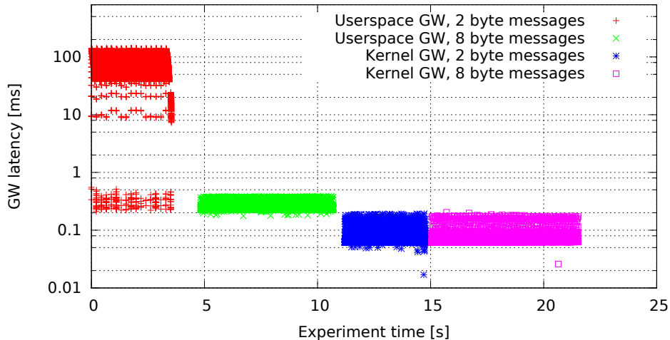
Single GW rule for all messages, no modifications (GW kernel 3.0.4-rt14-00008-gb2052fd, Traffic 50, Load none)
